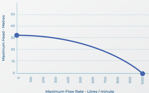
MH30-2 PUMP PERFORMANCE CURVE
